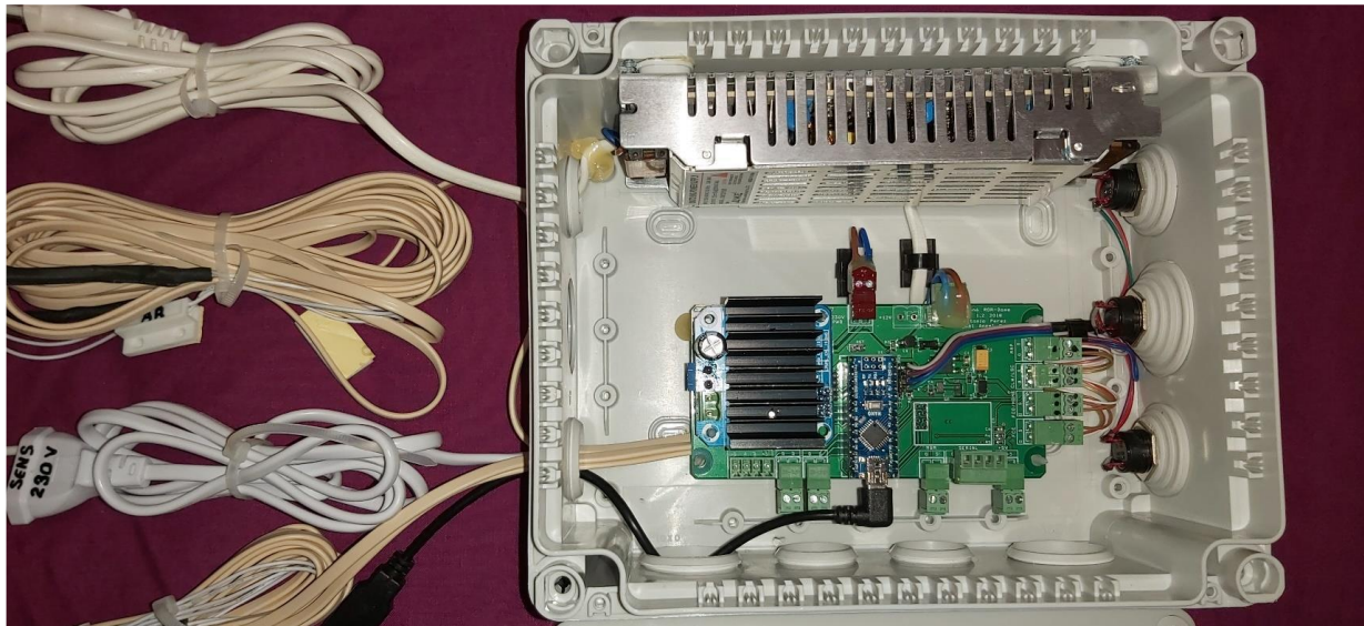
Controller with finished internal wiring
